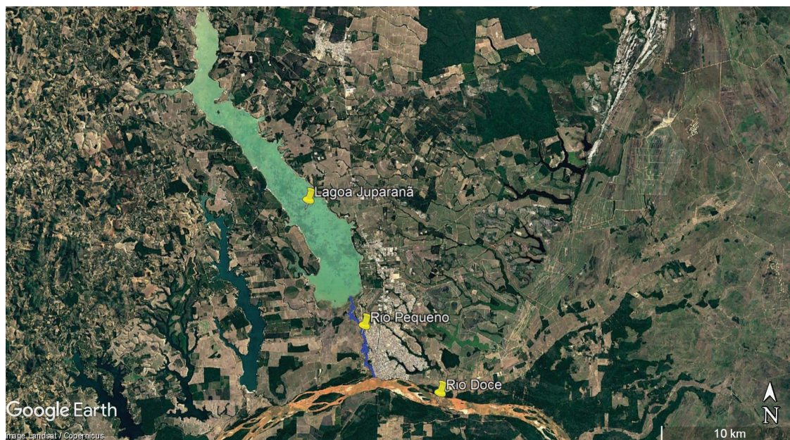
Figure 1a. View of the lower Rio Doce stretch and its marginal lakes. Lake Juparanã is shown in detail.
