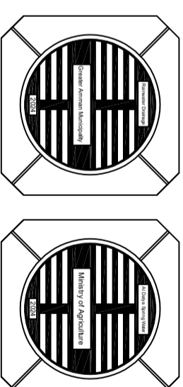
Detail.03 : Manhole cover detail
