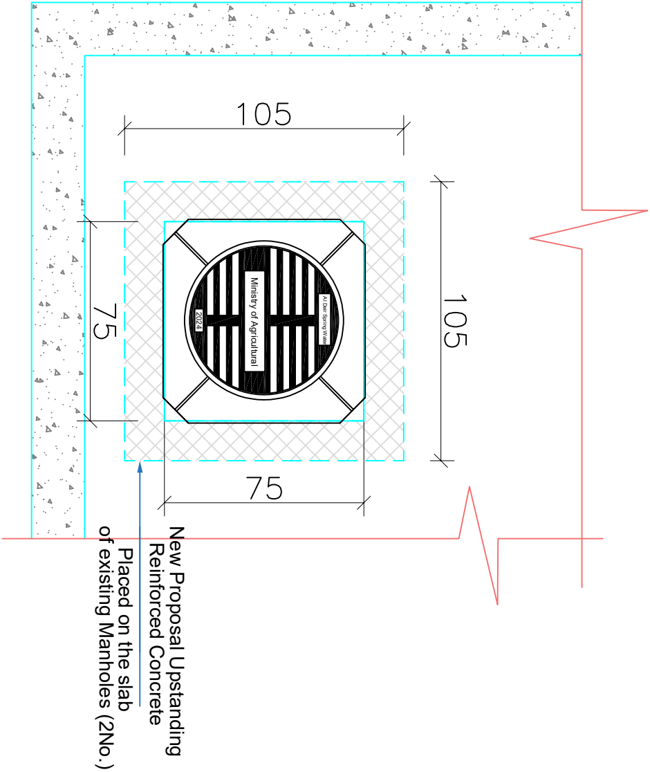
Designed Situation for Al Deir Manholes Available 2 Manholes
