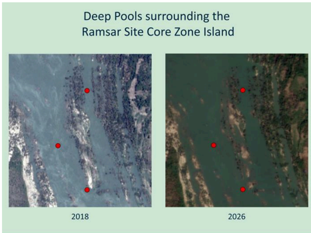
Figure 15: Locations of deep pools around the unnamed island east of Koh Phone Kep in 2018 and 2026
