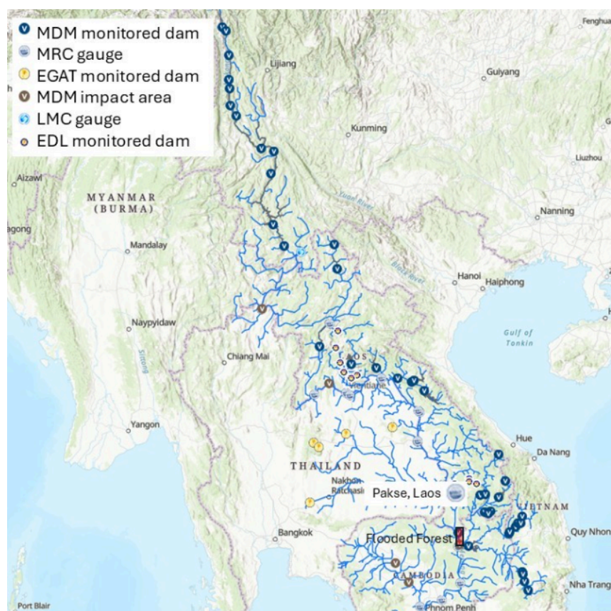
Figure 2: Location of large dams and reservoirs upstream of the STRS
