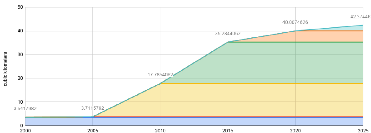
Figure 3: Cumulative Active Storage of Large Dams Upstream of Stung Treng Flooded Forest (2000-2025) (km³) Data: Mekong Dam Monitor
