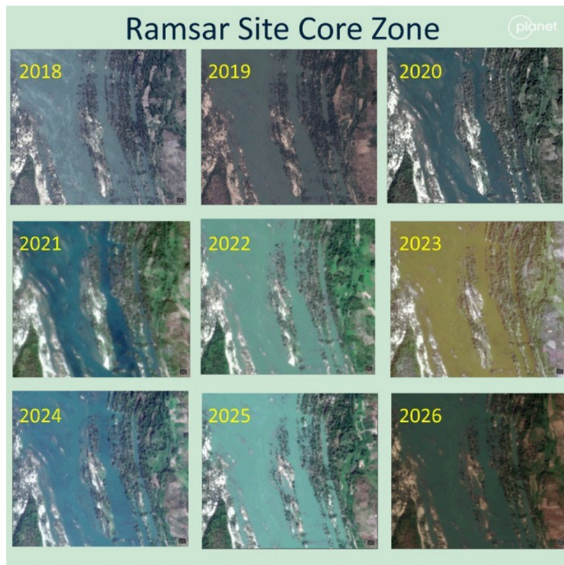
Figure 14: 2018-2026 visual timeline of change at the STRS Core Zone
