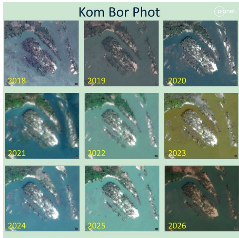
Figure 17: 2018-2026 visual timeline of change at Kom Bor Phot
