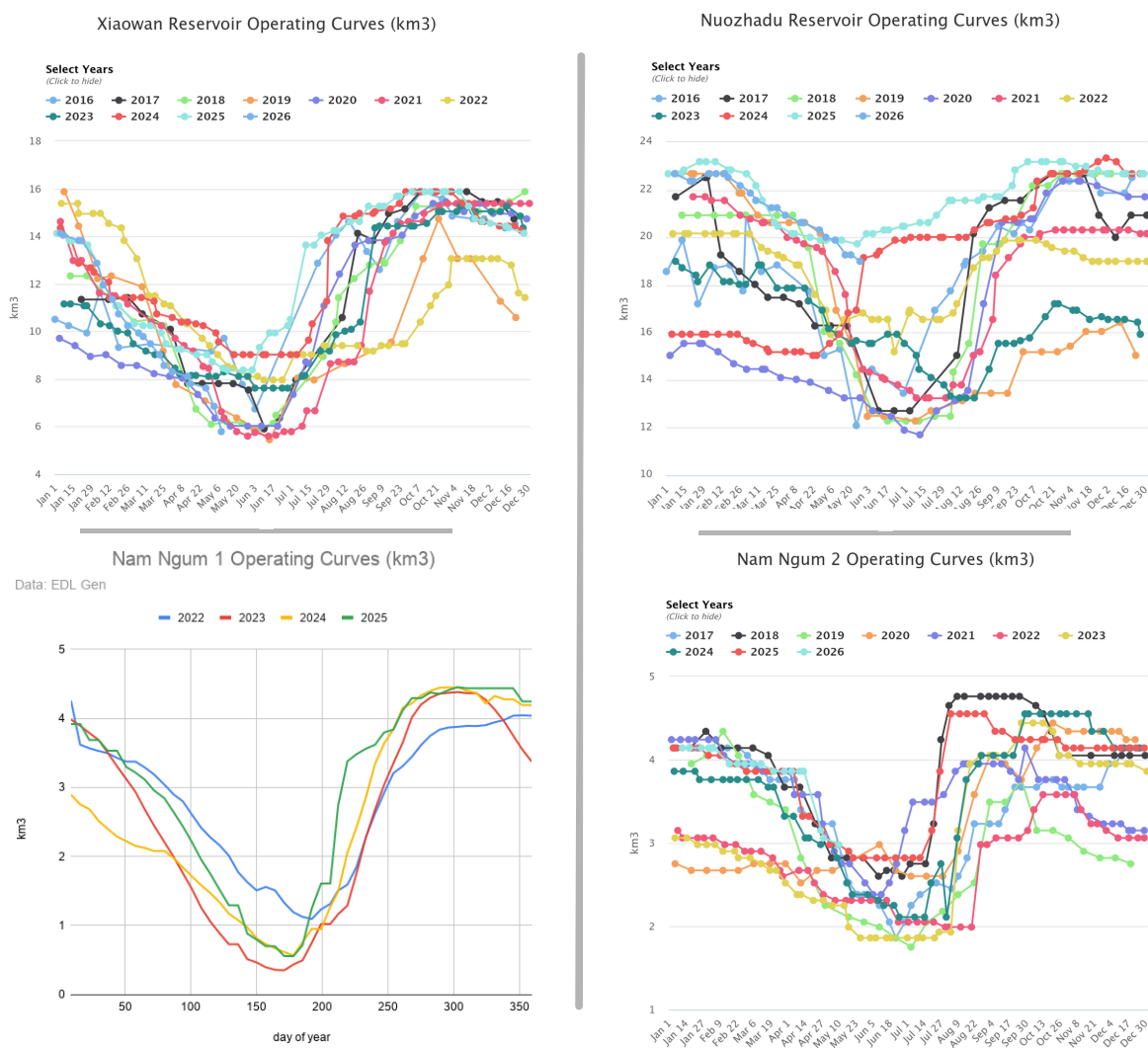
Figure 6: Estimated operating curves of the four largest dams upstream of flooded forest Source: Stimson Center, EDL-Gen
