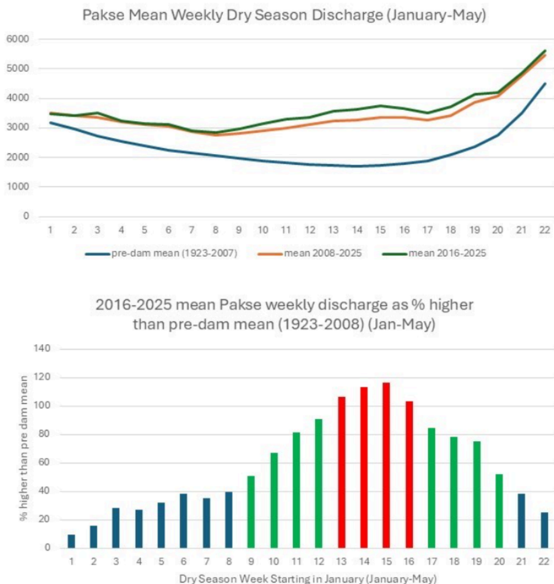
Figure 7: Pakse Discharge Analysis Source: Mekong River Commission
