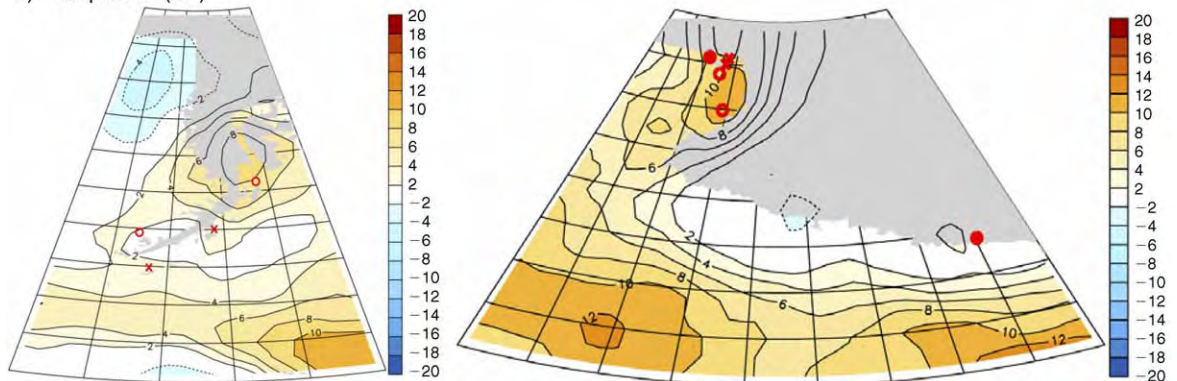
FIG. 7. ENSEMBLE model: simulated change in annual mean (a) zonal wind stress (note that due to the orientation of the figure a positive change means a greater stress directed toward the left/east of the figure); (b) surface air temperature; and (c) precipitation. Penguin colonies and the area shown in each panel are as in Fig. 6 (see also Figs. 1 and 2).
